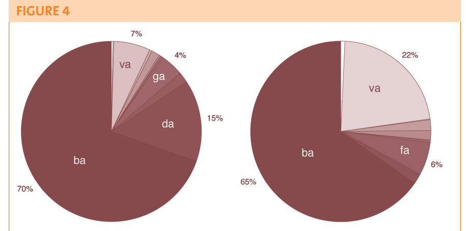
Figure 4: These pie charts show the proportion of confusions for two different /ba/ utterances, as reported by all of the 17 non-normal ears. The most common error for the /ba/ on the left is /da/ and then /va/, while the one on the right is most frequently heard as /va/ and then /fa/. The one on the left is almost never heard as /fa/ and the one on the right almost never as /da/. These two /ba/ sounds are reported correctly by normal ears.
