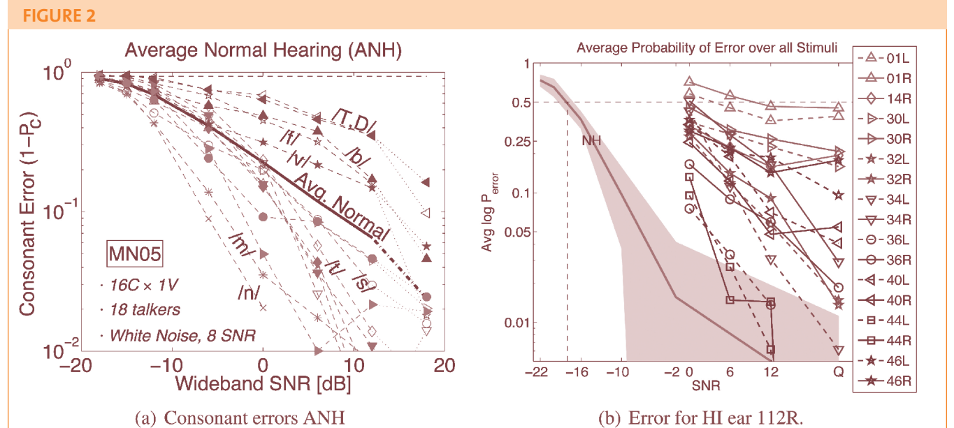
Figure 2. LEFT: Shown here is the average error (log scale) for 16 CV consonants as a function of the relative intensity of fllho-spectrum-level masking noise (Phatak et al., 2009). The solid black curve labeled “Avg. Normal” shows the average across all the consonants. Note the large variation in error. RIGHT: This family of curves compares the average consonant error (same as the black curve on the left) for 14 normal and 17 non-normal ears in speech shaped masking noise. For the non-normal ears, there is a large spread in scores due to the variation in hearing loss as compared to listeners with normal hearing (gray lines), all of whom are similar in their average performance.
