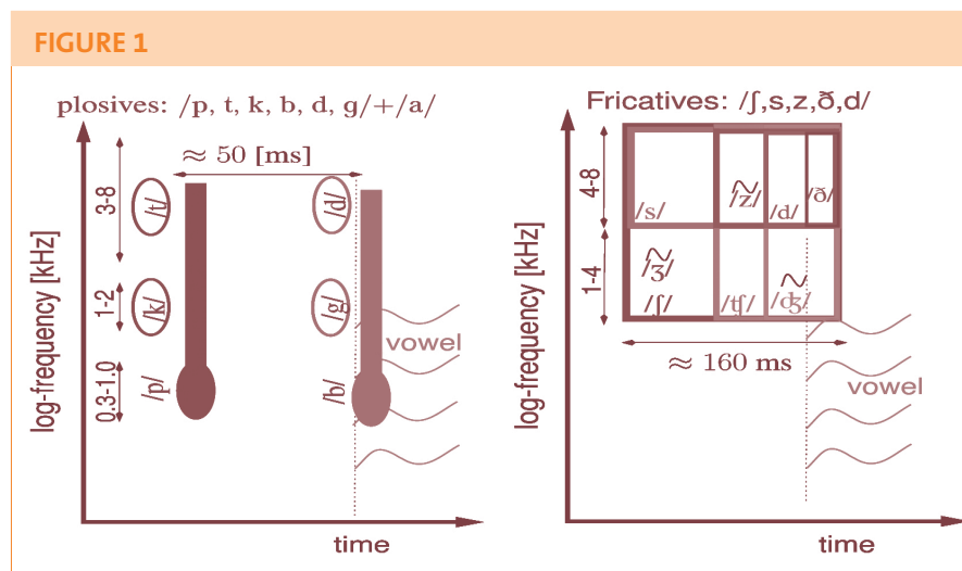
Figure 1. Time-frequency allocation of the plosives and the fricatives. Mapping these regions into perceptual cues required extensive perceptual experiments (Li et al., 2010). Once the sounds have been evaluated, it is possible to prove how the key noise-robust perceptual cues map to acoustic features. In the cases of the three voiced consonants indicated with a tilde ( /z, ʒ, dʒ/ ), the frication noise is modulated at the pitch frequency.
